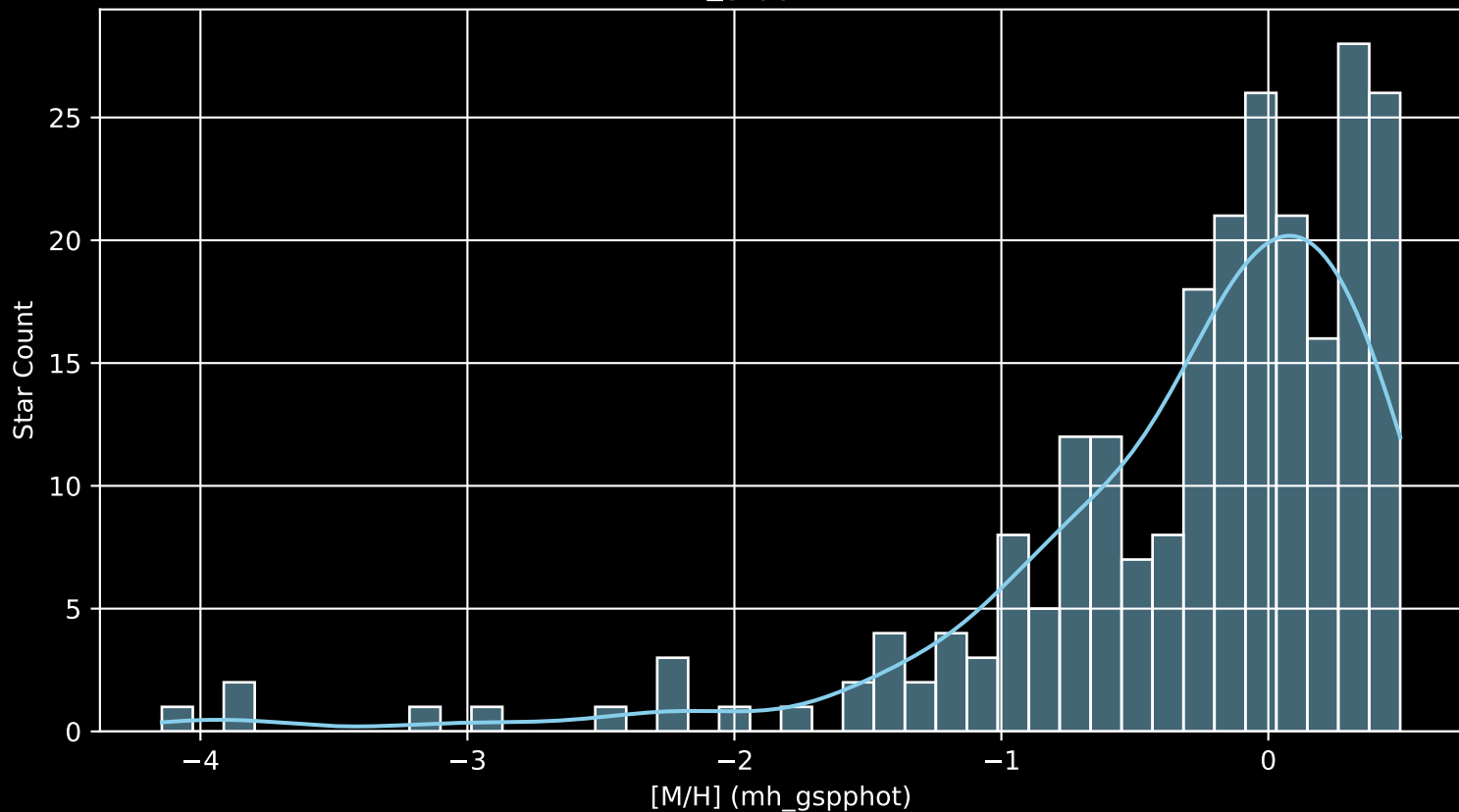
APOGEE DR17 Field: [000+04 [M/H] (mh_gspphot) (n= 234)
