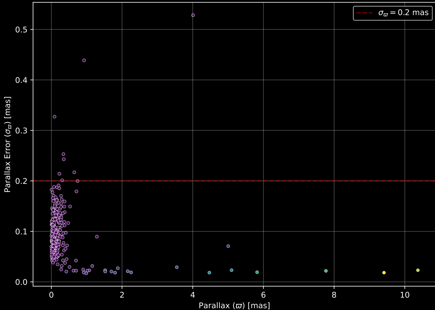
APOGEE DR17 Field: [000+04] Parallax Quality (n= 260)
