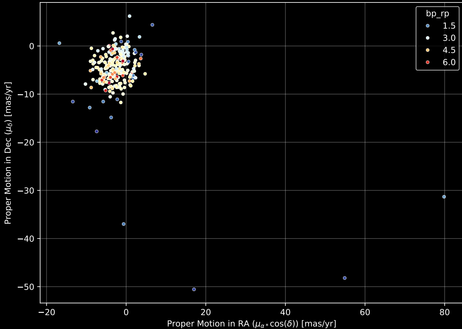
APOGEE DR17 Field: [000+04] Proper Motion Diagram (n= 260)
