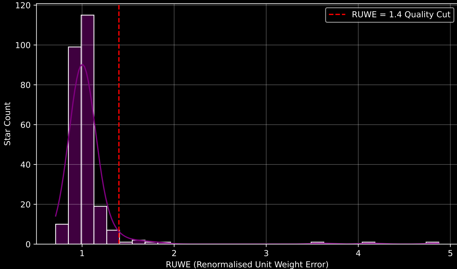
GAPOGEE DR17 Field [000+04] RUWE Distribution (n= 258)
